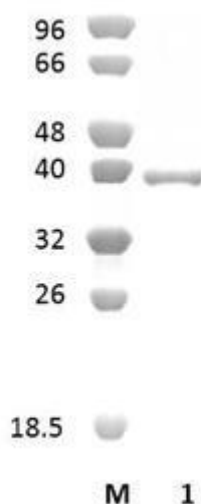
Figure 1. SDS-PAGE analysis of CcMan5B (GH5) was conducted in (Lane 1), employing a 14% polyacrylamide gel. The enzyme exhibits a band corresponding to a molecular weight of approximately 39,29 kDa. Lane M contains a Protein Marker for reference.
