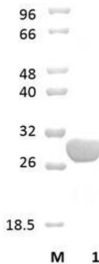
Figure 1. SDS-PAGE analysis of CBM78 was conducted in (Lane 1), employing a 14% polyacrylamide gel. The enzyme exhibits a band corresponding to a molecular weight of approximately 23,04 kDa. Lane M contains a Protein Marker for reference.
