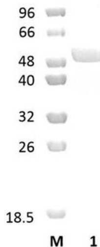
Figure 1. SDS-PAGE analysis of BfNan33A (GH33) was conducted in (Lane 1), employing a 14% polyacrylamide gel. The enzyme exhibits a band corresponding to a molecular weight of approximately 54,42 kDa. Lane M contains a Protein Marker for reference.
