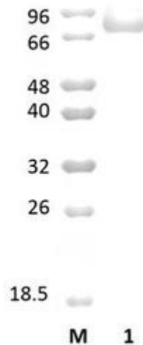
Figure 1. SDS-PAGE analysis of BoXyn98A (GH98-CBM35) was conducted in (Lane 1), employing a 14% polyacrylamide gel. The enzyme exhibits a band corresponding to a molecular weight of approximately 84,53 kDa. Lane M contains a Protein Marker for reference.
