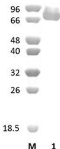
Figure 1. SDS-PAGE analysis of BoGlc67A (GH67) was conducted in (Lane 1), employing a 14% polyacrylamide gel. The enzyme exhibits a band corresponding to a molecular weight of approximately 82,46 kDa. Lane M contains a Protein Marker for reference.
