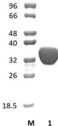
Figure 1. SDS-PAGE analysis of PpGlt17A (GH17) was conducted in (Lane 1), employing a 14% polyacrylamide gel. The enzyme exhibits a band corresponding to a molecular weight of approximately 36,38 kDa. Lane M contains a Protein Marker for reference.
