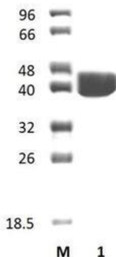
Figure 1. SDS-PAGE analysis of PpXgh5A (GH5) was conducted in (Lane 1), employing a 14% polyacrylamide gel. The enzyme exhibits a band corresponding to a molecular weight of approximately 45,15 kDa. Lane M contains a Protein Marker for reference.
