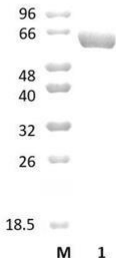
Figure 1. SDS-PAGE analysis of PpEbd9A (GH9) was conducted in (Lane 1), employing a 14% polyacrylamide gel. The enzyme exhibits a band corresponding to a molecular weight of approximately 70,12 kDa. Lane M contains a Protein Marker for reference.
