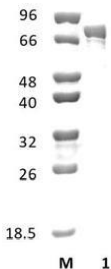
Figure 1. SDS-PAGE analysis of TsXyl120A (GH120) was conducted in (Lane 1), employing a 14% polyacrylamide gel. The enzyme exhibits a band corresponding to a molecular weight of approximately 75,91 kDa. Lane M contains a Protein Marker for reference.
