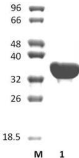
Figure 1. SDS-PAGE analysis of BpAga16A (GH16) was conducted in (Lane 1), employing a 14% polyacrylamide gel. The enzyme exhibits a band corresponding to a molecular weight of approximately 37,99 kDa. Lane M contains a Protein Marker for reference.
