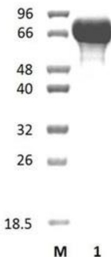
Figure 1. SDS-PAGE analysis of Bb Nga129A (GH129) was conducted in (Lane 1), employing a 14% polyacrylamide gel. The enzyme exhibits a band corresponding to a molecular weight of approximately 75,94 kDa. Lane M contains a Protein Marker for reference.
