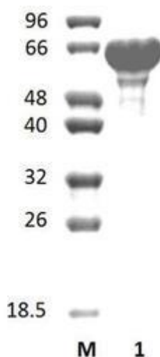
Figure 1. SDS-PAGE analysis of ABff68A (GH68) was conducted in (Lane 1), employing a 14% polyacrylamide gel. The enzyme exhibits a band corresponding to a molecular weight of approximately 63,98 kDa. Lane M contains a Protein Marker for reference.
