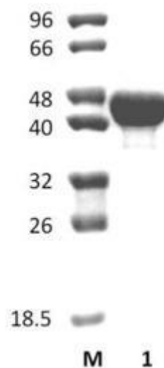
Figure 1. SDS-PAGE analysis of BcAmy14A (GH14) was conducted in (Lane 1), employing a 14% polyacrylamide gel. The enzyme exhibits a band corresponding to a molecular weight of approximately 47,04 kDa. Lane M contains a Protein Marker for reference.
