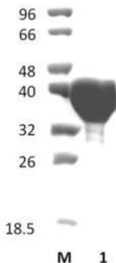
Figure 1. SDS-PAGE analysis of BcMan76A (GH76) was conducted in (Lane 1), employing a 14% polyacrylamide gel. The enzyme exhibits a band corresponding to a molecular weight of approximately 41,79 kDa. Lane M contains a Protein Marker for reference.
