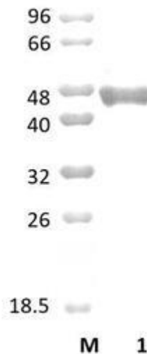
Figure 1. SDS-PAGE analysis of BcAmy14B (GH14) was conducted in (Lane 1), employing a 14% polyacrylamide gel. The enzyme exhibits a band corresponding to a molecular weight of approximately 48,23 kDa. Lane M contains a Protein Marker for reference.
