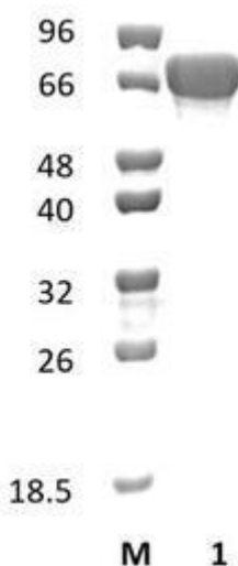
Figure 1. SDS-PAGE analysis of BsLac42A (GH42) was conducted in (Lane 1), employing a 14% polyacrylamide gel. The enzyme exhibits a band corresponding to a molecular weight of approximately 82,26 kDa. Lane M contains a Protein Marker for reference.
