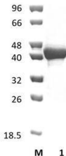
Figure 1. SDS-PAGE analysis of TmXyn10A (GH10) was conducted in (Lane 1), employing a 14% polyacrylamide gel. The enzyme exhibits a band corresponding to a molecular weight of approximately 43,30 kDa. Lane M contains a Protein Marker for reference.
