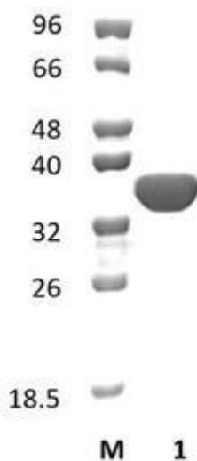
Figure 1. SDS-PAGE analysis of BMan5A (GH5) was conducted in (Lane 1), employing a 14% polyacrylamide gel. The enzyme exhibits a band corresponding to a molecular weight of approximately 35,51 kDa. Lane M contains a Protein Marker for reference.
