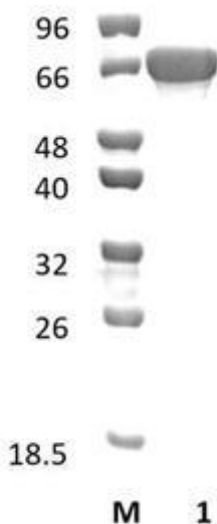
Figure 1. SDS-PAGE analysis of BfDex49A (GH49) was conducted in (Lane 1), employing a 14% polyacrylamide gel. The enzyme exhibits a band corresponding to a molecular weight of approximately 70,95 kDa. Lane M contains a Protein Marker for reference.
