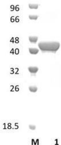
Figure 1. SDS-PAGE analysis of TtGe15B (CE15) was conducted in (Lane 1), employing a 14% polyacrylamide gel. The enzyme exhibits a band corresponding to a molecular weight of approximately 42,35 kDa. Lane M contains a Protein Marker for reference.
