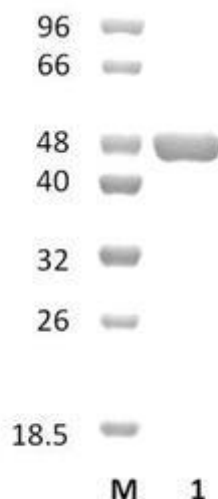
Figure 1. SDS-PAGE analysis of ZgGe15A (CE15) was conducted in (Lane 1), employing a 14% polyacrylamide gel. The enzyme exhibits a band corresponding to a molecular weight of approximately 47,24 kDa. Lane M contains a Protein Marker for reference.
