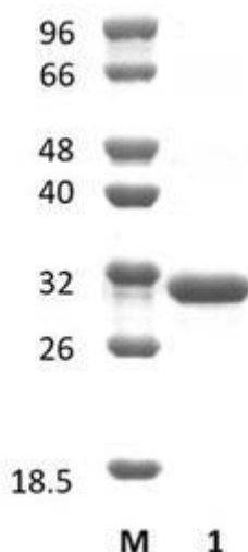
Figure 1. SDS-PAGE analysis of CsFae1A (CE1) was conducted in (Lane 1), employing a 14% polyacrylamide gel. The enzyme exhibits a band corresponding to a molecular weight of approximately 30,95 kDa. Lane M contains a Protein Marker for reference.
