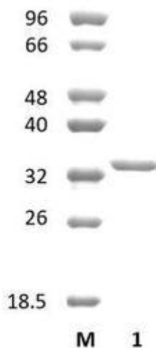
Figure 1. SDS-PAGE analysis of UbFae1B (CE1) was conducted in (Lane 1), employing a 14% polyacrylamide gel. The enzyme exhibits a band corresponding to a molecular weight of approximately 33,12 kDa. Lane M contains a Protein Marker for reference.
