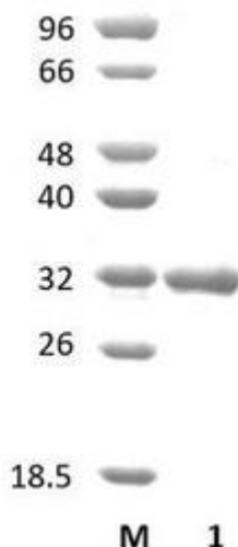
Figure 1. SDS-PAGE analysis of PmFae1A (CE1) was conducted in (Lane 1), employing a 14% polyacrylamide gel. The enzyme exhibits a band corresponding to a molecular weight of approximately 32,44 kDa. Lane M contains a Protein Marker for reference.
