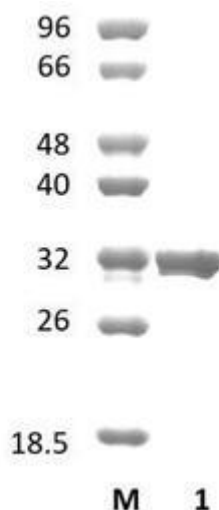
Figure 1. SDS-PAGE analysis of BfFae1B (CE1) was conducted in (Lane 1), employing a 14% polyacrylamide gel. The enzyme exhibits a band corresponding to a molecular weight of approximately 31,33 kDa. Lane M contains a Protein Marker for reference.
