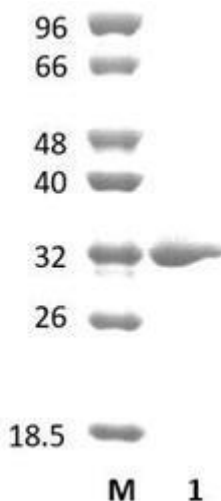
Figure 1. SDS-PAGE analysis of PtFae1A (CE1) was conducted in (Lane 1), employing a 14% polyacrylamide gel. The enzyme exhibits a band corresponding to a molecular weight of approximately 32,52 kDa. Lane M contains a Protein Marker for reference.
