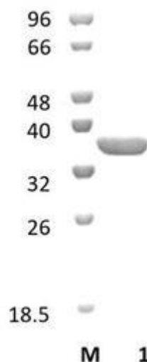
Figure 1. SDS-PAGE analysis of MmFae1B (CE1) was conducted in (Lane 1), employing a 14% polyacrylamide gel. The enzyme exhibits a band corresponding to a molecular weight of approximately 35,36 kDa. Lane M contains a Protein Marker for reference.
