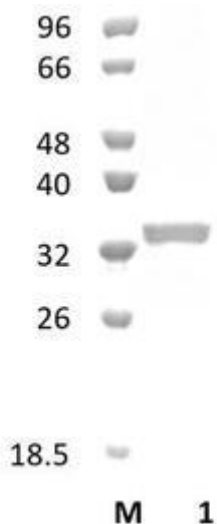
Figure 1. SDS-PAGE analysis of KpFae1A (CE1) was conducted in (Lane 1), employing a 14% polyacrylamide gel. The enzyme exhibits a band corresponding to a molecular weight of approximately 36,55 kDa. Lane M contains a Protein Marker for reference.
