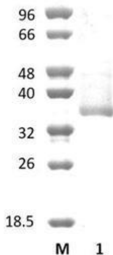
Figure 1. SDS-PAGE analysis of MkFae1A (CE1) was conducted in (Lane 1), employing a 14% polyacrylamide gel. The enzyme exhibits a band corresponding to a molecular weight of approximately 35,90 kDa. Lane M contains a Protein Marker for reference.
