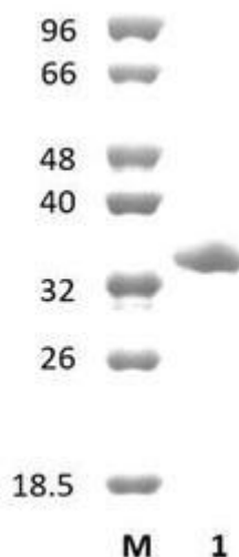
Figure 1. SDS-PAGE analysis of BpFae1B (CE1) was conducted in (Lane 1), employing a 14% polyacrylamide gel. The enzyme exhibits a band corresponding to a molecular weight of approximately 34,57 kDa. Lane M contains a Protein Marker for reference.
