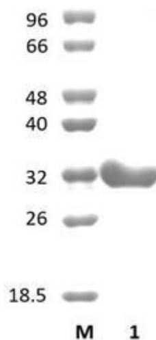
Figure 1. SDS-PAGE analysis of LhFae1A (CE1) was conducted in (Lane 1), employing a 14% polyacrylamide gel. The enzyme exhibits a band corresponding to a molecular weight of approximately 29,70 kDa. Lane M contains a Protein Marker for reference.
