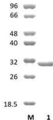
Figure 1. SDS-PAGE analysis of SdFae1A (CE1) was conducted in (Lane 1), employing a 14% polyacrylamide gel. The enzyme exhibits a band corresponding to a molecular weight of approximately 29,84 kDa. Lane M contains a Protein Marker for reference.
