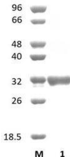
Figure 1. SDS-PAGE analysis of UbFae1C (CE1) was conducted in (Lane 1), employing a 14% polyacrylamide gel. The enzyme exhibits a band corresponding to a molecular weight of approximately 30,88 kDa. Lane M contains a Protein Marker for reference.
