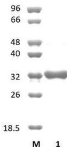
Figure 1. SDS-PAGE analysis of TmFae1A (CE1) was conducted in (Lane 1), employing a 14% polyacrylamide gel. The enzyme exhibits a band corresponding to a molecular weight of approximately 31,30 kDa. Lane M contains a Protein Marker for reference.
