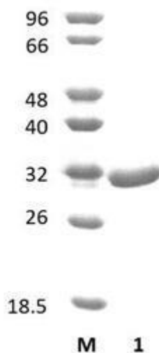
Figure 1. SDS-PAGE analysis of LcFae1A (CE1) was conducted in (Lane 1), employing a 14% polyacrylamide gel. The enzyme exhibits a band corresponding to a molecular weight of approximately 29,79 kDa. Lane M contains a Protein Marker for reference.
