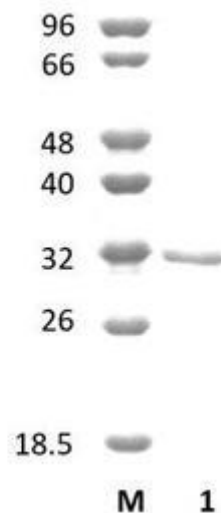
Figure 1. SDS-PAGE analysis of PtFae1C (CE1) was conducted in (Lane 1), employing a 14% polyacrylamide gel. The enzyme exhibits a band corresponding to a molecular weight of approximately 30,89 kDa. Lane M contains a Protein Marker for reference.
