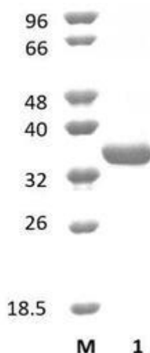
Figure 1. SDS-PAGE analysis of AbFae1A (CE1) was conducted in (Lane 1), employing a 14% polyacrylamide gel. The enzyme exhibits a band corresponding to a molecular weight of approximately 35,12 kDa. Lane M contains a Protein Marker for reference.
