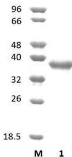
Figure 1. SDS-PAGE analysis of BFae1C (CE1) was conducted in (Lane 1), employing a 14% polyacrylamide gel. The enzyme exhibits a band corresponding to a molecular weight of approximately 31,31 kDa. Lane M contains a Protein Marker for reference.
