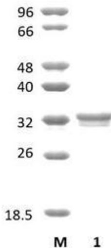
Figure 1. SDS-PAGE analysis of BpFae1A (CE1) was conducted in (Lane 1), employing a 14% polyacrylamide gel. The enzyme exhibits a band corresponding to a molecular weight of approximately 32,53 kDa. Lane M contains a Protein Marker for reference.
