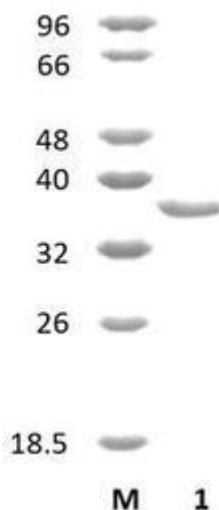
Figure 1. SDS-PAGE analysis of B/Fae1A (CE1) was conducted in (Lane 1), employing a 14% polyacrylamide gel. The enzyme exhibits a band corresponding to a molecular weight of approximately 36,42 kDa. Lane M contains a Protein Marker for reference.
