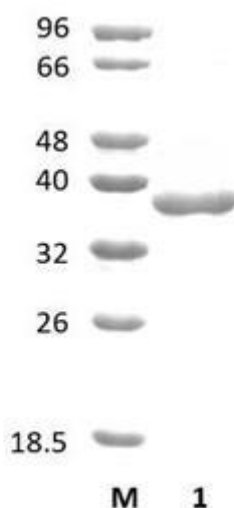
Figure 1. SDS-PAGE analysis of FFae1A (CE1) was conducted in (Lane 1), employing a 14% polyacrylamide gel. The enzyme exhibits a band corresponding to a molecular weight of approximately 35,40 kDa. Lane M contains a Protein Marker for reference.
