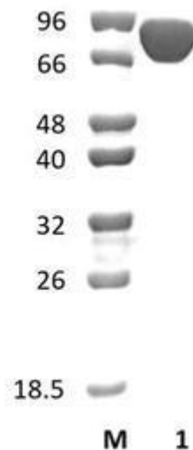
Figure 1. SDS-PAGE analysis of CbCel48A (GH48) was conducted in (Lane 1), employing a 14% polyacrylamide gel. The enzyme exhibits a band corresponding to a molecular weight of approximately 76,49 kDa. Lane M contains a Protein Marker for reference.
