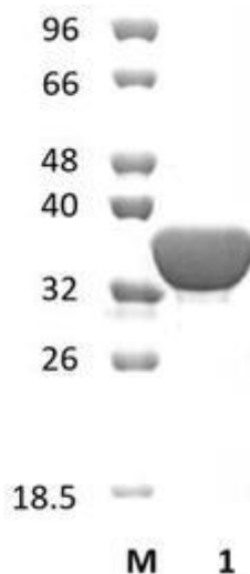
Figure 1. SDS-PAGE analysis of MsGpi14A (CE14) was conducted in (Lane 1), employing a 14% polyacrylamide gel. The enzyme exhibits a band corresponding to a molecular weight of approximately 35,44 kDa. Lane M contains a Protein Marker for reference.
