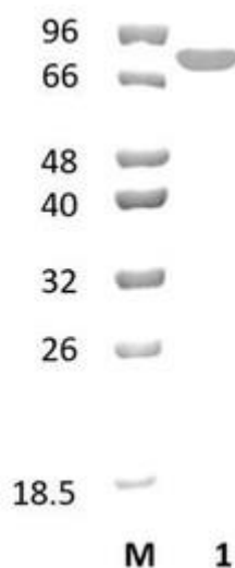
Figure 1. SDS-PAGE analysis of SdMal77A (GH77) was conducted in (Lane 1), employing a 14% polyacrylamide gel. The enzyme exhibits a band corresponding to a molecular weight of approximately 83,25 kDa. Lane M contains a Protein Marker for reference.
