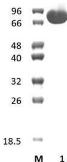
Figure 1. SDS-PAGE analysis of GsAgu67A (GH67) was conducted in (Lane 1), employing a 14% polyacrylamide gel. The enzyme exhibits a band corresponding to a molecular weight of approximately 80,45 kDa. Lane M contains a Protein Marker for reference.
