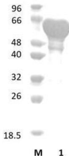
Figure 1. SDS-PAGE analysis of SpEab98A (GH98) was conducted in (Lane 1), employing a 14% polyacrylamide gel. The enzyme exhibits a band corresponding to a molecular weight of approximately 67,45 kDa. Lane M contains a Protein Marker for reference.
