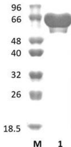
Figure 1. SDS-PAGE analysis of BpPor86A (GH86) was conducted in (Lane 1), employing a 14% polyacrylamide gel. The enzyme exhibits a band corresponding to a molecular weight of approximately 66,68 kDa. Lane M contains a Protein Marker for reference.
