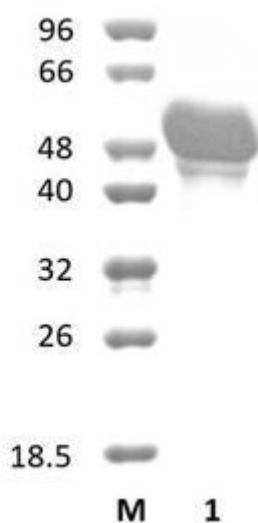
Figure 1. SDS-PAGE analysis of BoAga50A (GH50) was conducted in (Lane 1), employing a 14% polyacrylamide gel. The enzyme exhibits a band corresponding to a molecular weight of approximately 53,68 kDa. Lane M contains a Protein Marker for reference.
