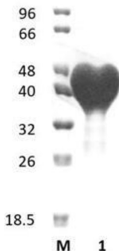
Figure 1. SDS-PAGE analysis of SdAhg117A (GH117) was conducted in (Lane 1), employing a 14% polyacrylamide gel. The enzyme exhibits a band corresponding to a molecular weight of approximately 43,53 kDa. Lane M contains a Protein Marker for reference.
