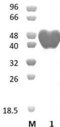
Figure 1. SDS-PAGE analysis of BeXyn5A (GH5) was conducted in (Lane 1), employing a 14% polyacrylamide gel. The enzyme exhibits a band corresponding to a molecular weight of approximately 47,96 kDa. Lane M contains a Protein Marker for reference.
